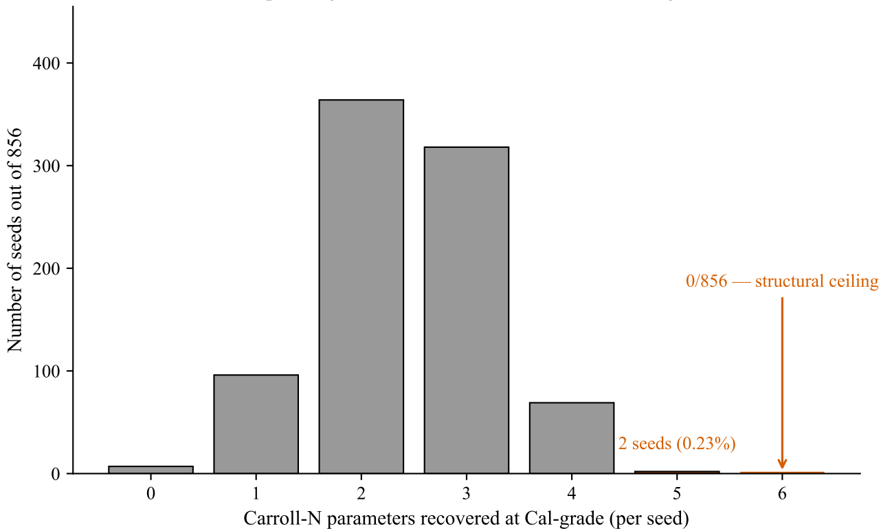
v3.1 sweep: Cal-grade distribution (856 seeds, 86 configurations)
