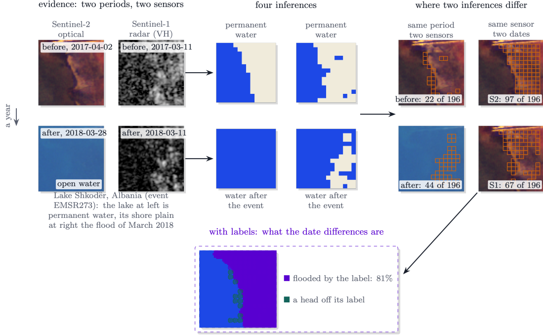
Figure 3: Four dated inputs of one GEOID-Flood chip, each read on identical windows: the same-period and same-sensor differences on the scene, with the comparison against labels shown separately.
