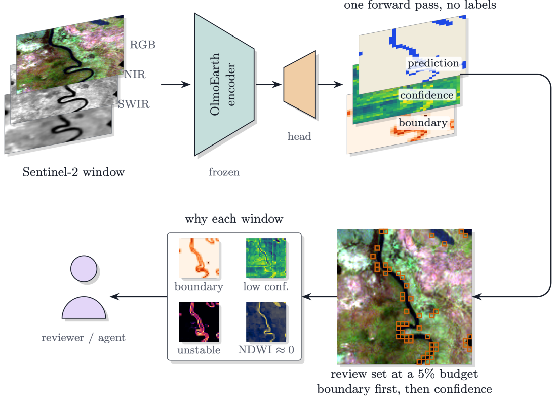
Figure 2: One scene through the label-free assessment: Sentinel-2 bands, the frozen OlmoEarth encoder and a task head, the prediction with its confidence and boundary layers, the review set at a 5% budget, and the cues per flagged window.
