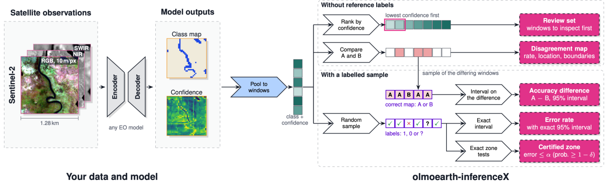
Figure 1: The structure of the package. It reads a model’s class scores (and optionally a second map and a raster of input conditions), pools them to windows that each carry a class and the model’s confidence, and answers two kinds of question. Without labels, it ranks the windows by confidence into a review set (Section 2.1) and compares two maps (Section 2.2). With a labelled sample, windows drawn at random give the error rate with an exact interval (Section 2.3) and, by exact tests on the most confident zones, a certified zone (Section 2.4); windows drawn where two maps differ give the accuracy difference (Section 2.5). Each step runs per input condition when a condition raster is given.
