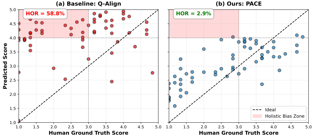
Figure 5: Holistic Bias on Prominent Dimensions ( Tactile Satisfaction & Human Vitality ) . On highly specific and challenging dimensions, direct MLLM prompting (Q-Align) suffers a catastrophic HOR of 58.8%, showing strong interference from holistic aesthetic priors during task-specific reasoning. PACE maintains robust evidence-based scoring (2.9% HOR).
