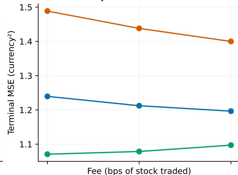
252 days; strike/forward 1.1
