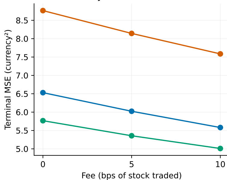
252 days; strike/forward 1.0
