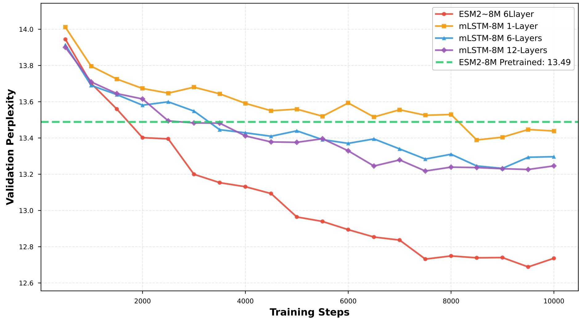
Depth Comparison (LR=1e-3, Warmup=2000)
