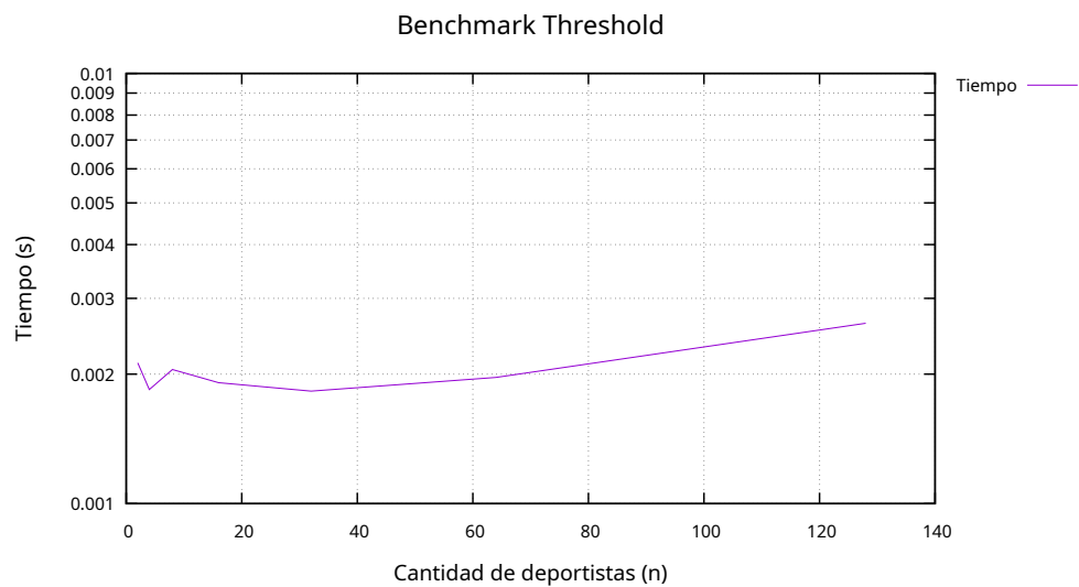
Figura 5.10: Benchmark de threshold
