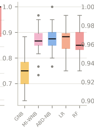
synth-conflict
