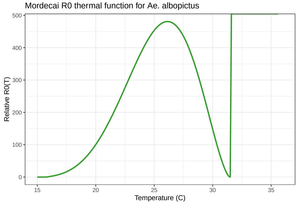
Figure 10: Mordecai R0 thermal functions
