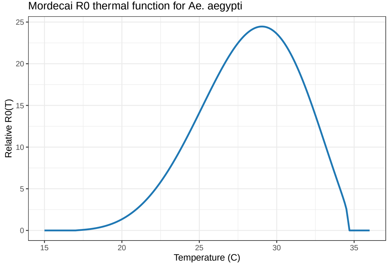
Figure 9: Mordecai R0 thermal functions
