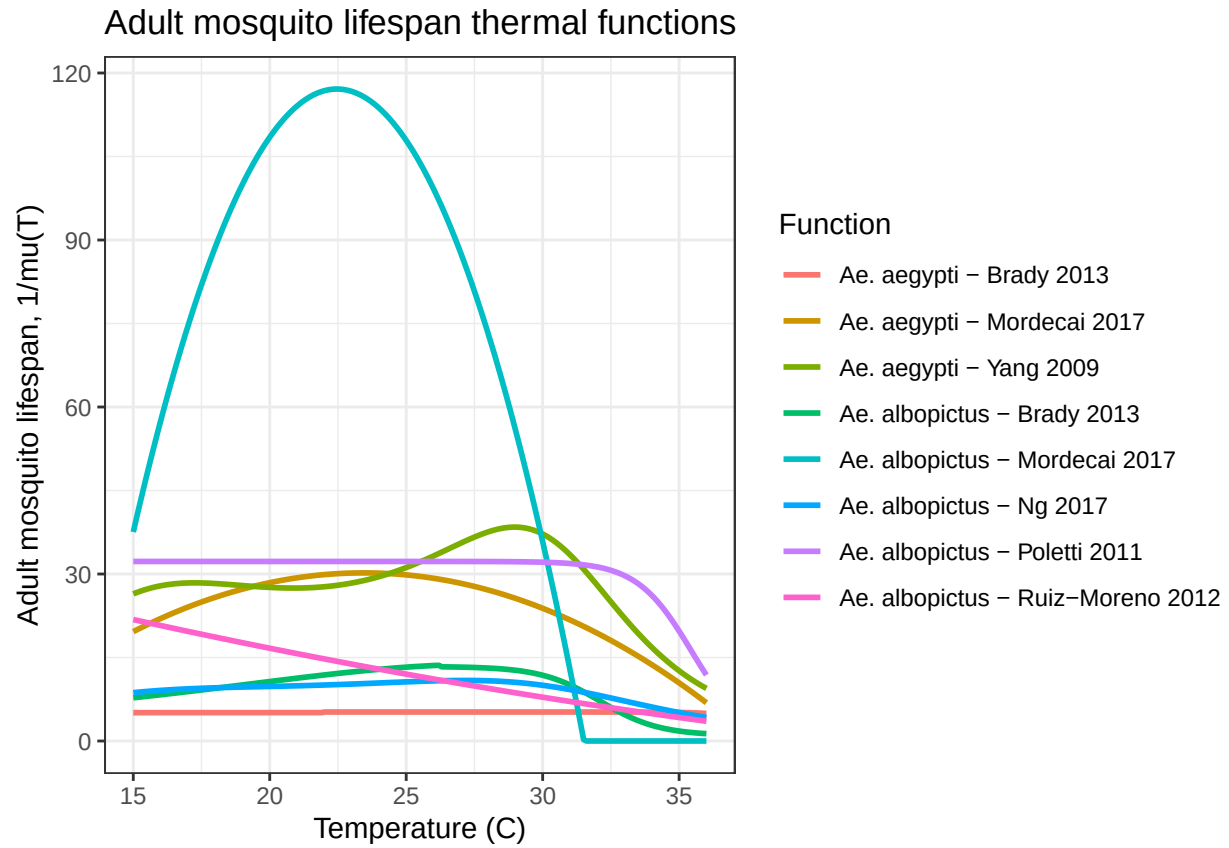
Figure 4: Adult mosquito lifespan thermal functions
