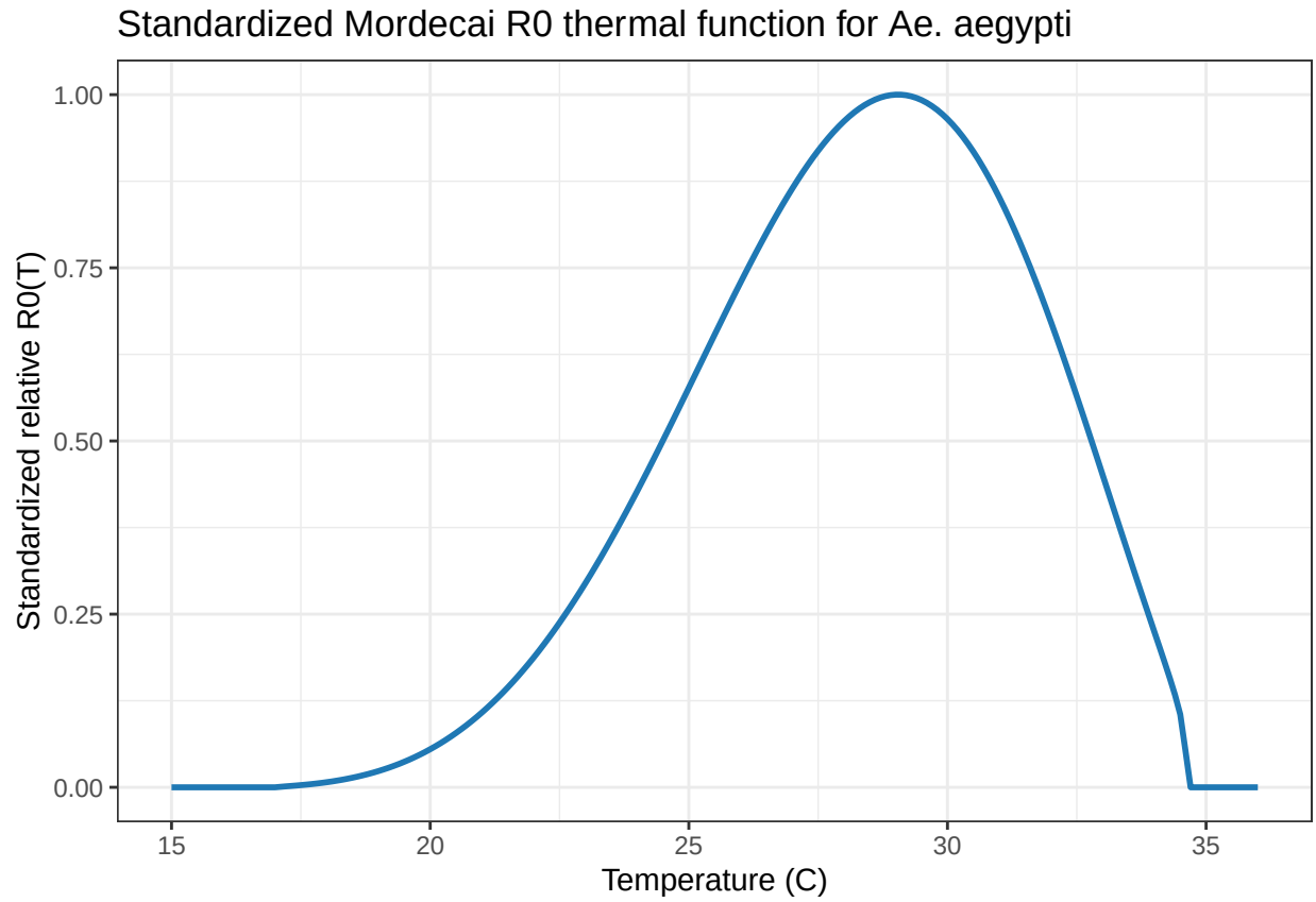
Figure 9: Mordecai R0 thermal functions
