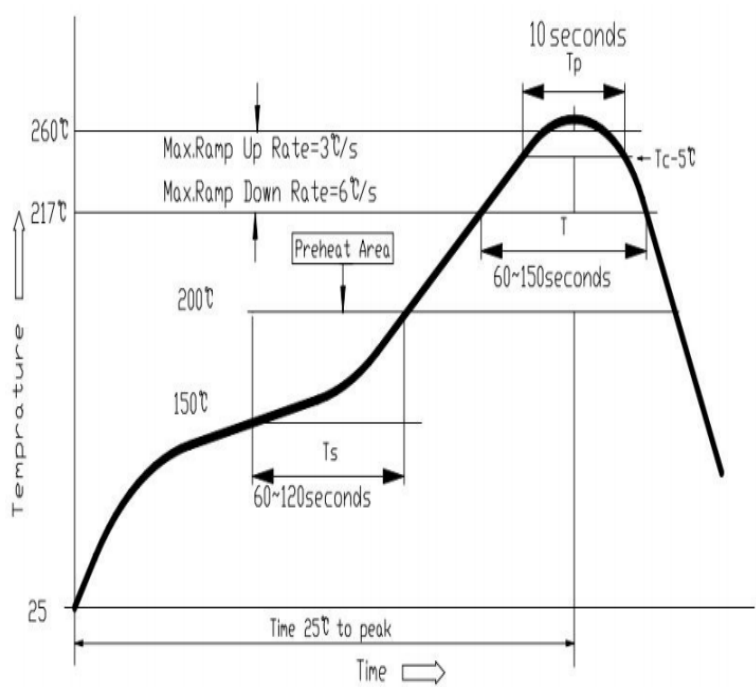
Figure 1. Re-flow Soldering (Lead Free)
