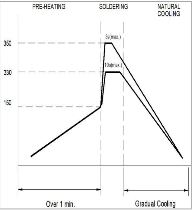
Figure 2. Hand Soldering
