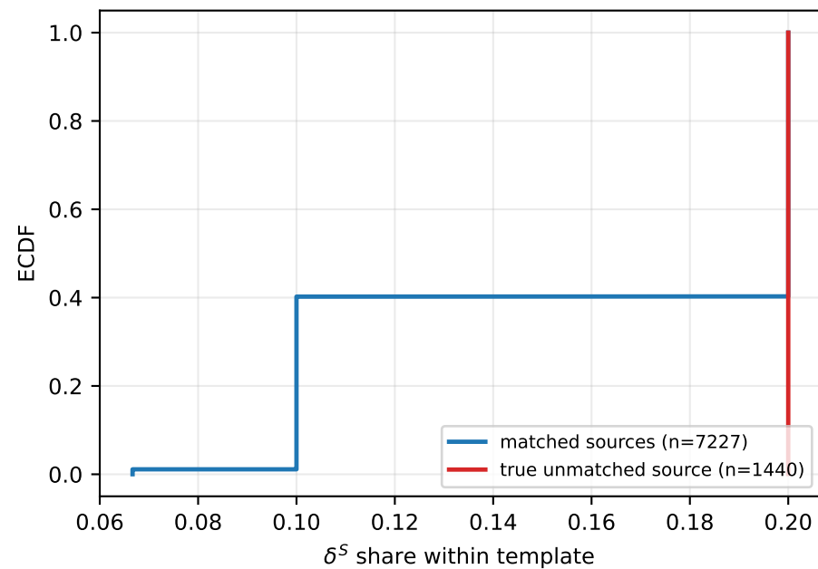
(a) Source unmatched-mass share
