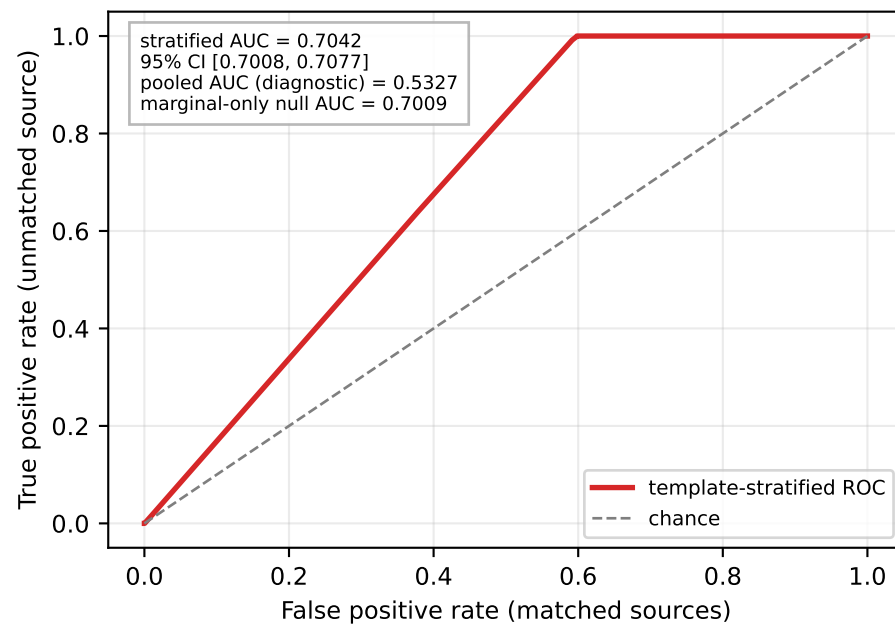
(b) Discrimination (not calibration)
