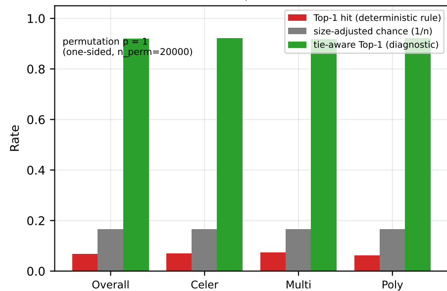
(c) Source Top-1 localization
