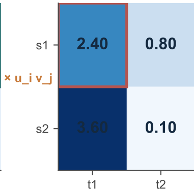
(b) Raw plan P = \text{diag}(u)K \text{diag}(v) destination scaling v = (4, 1)
