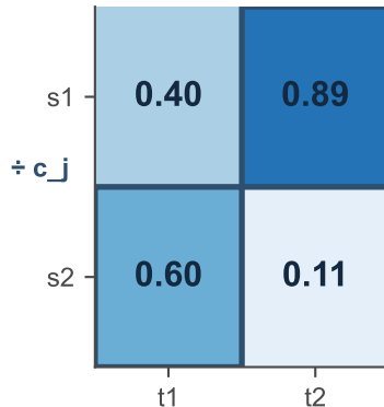
(c) Conditional scores S\_row = P / c c1 = 6.0, c2 = 0.9
