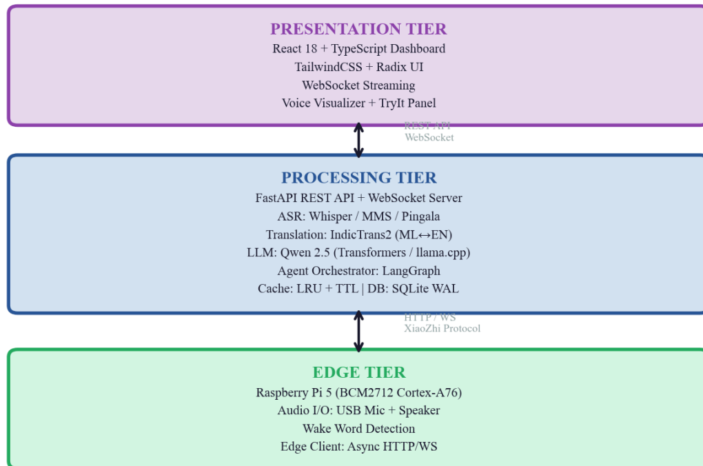
Fig 3.1a — Three-Tier System Architecture
