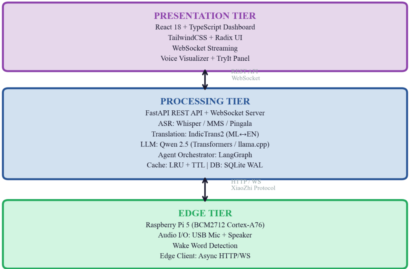
Fig 3.1a — Three-Tier System Architecture
