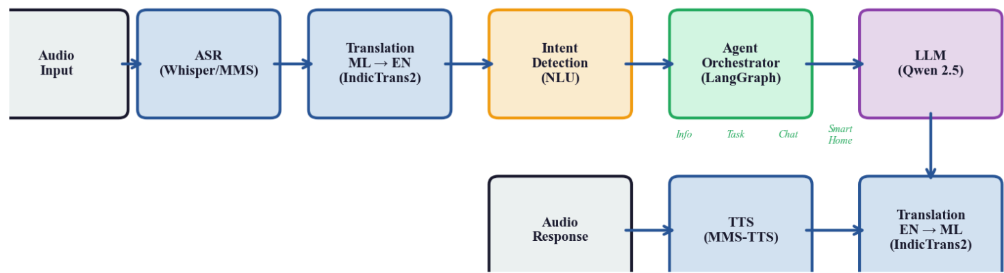
Fig 3.2 — End-to-End Voice Processing Pipeline
