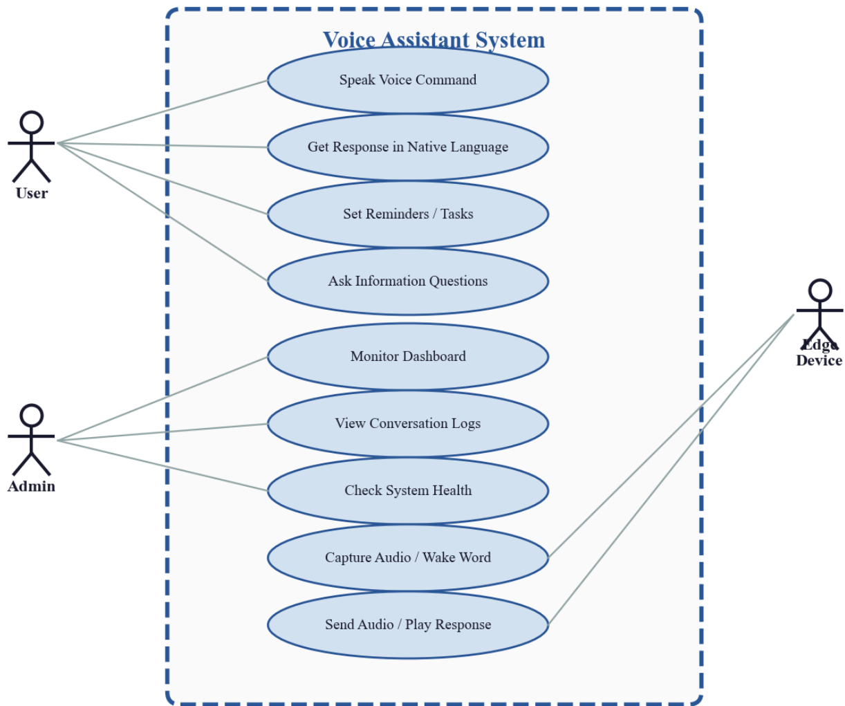
Fig 3.3 — Use-Case Diagram
