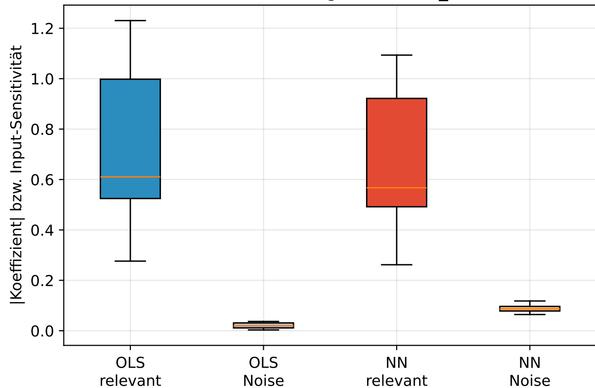
Relevante vs. Noise-Regressoren (n_noise=25)
