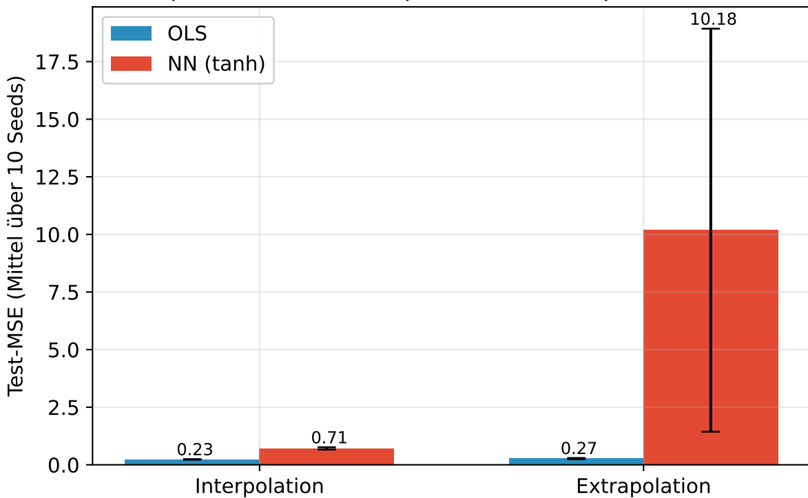
Interpolations- vs. Extrapolationsfehler (p=5, 10 Seeds)
