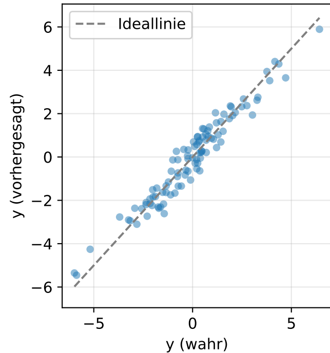
identity (MSE=0.271)
