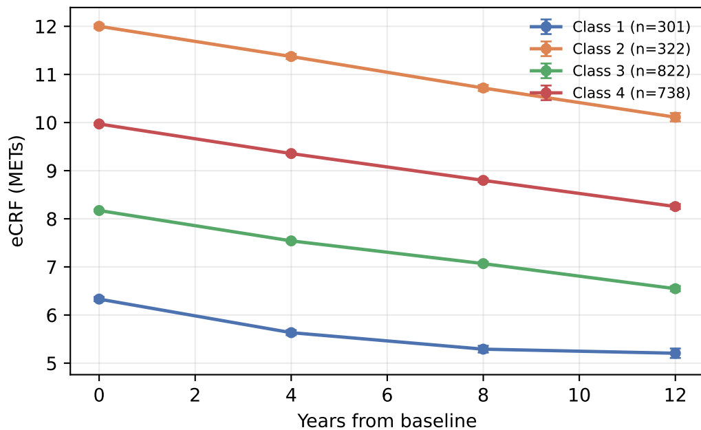
HRS (even waves, 2006-2018)
