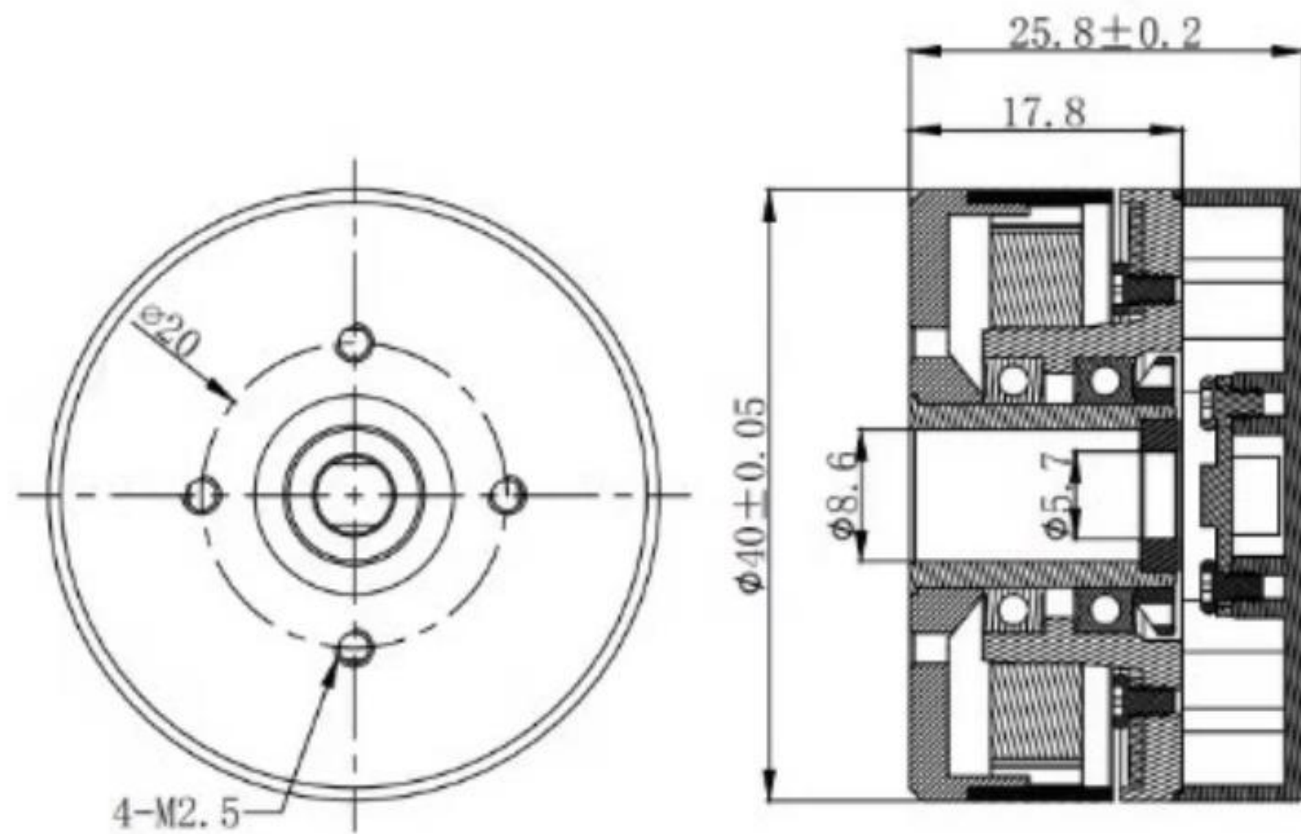
GM3506 w/Encoder
