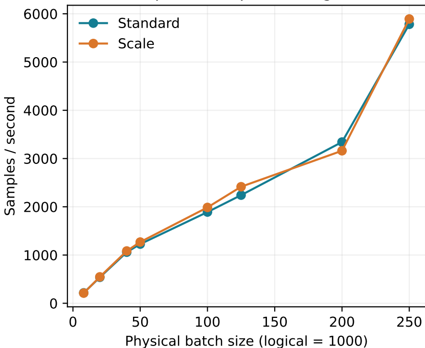
Complete DP update, length 64
