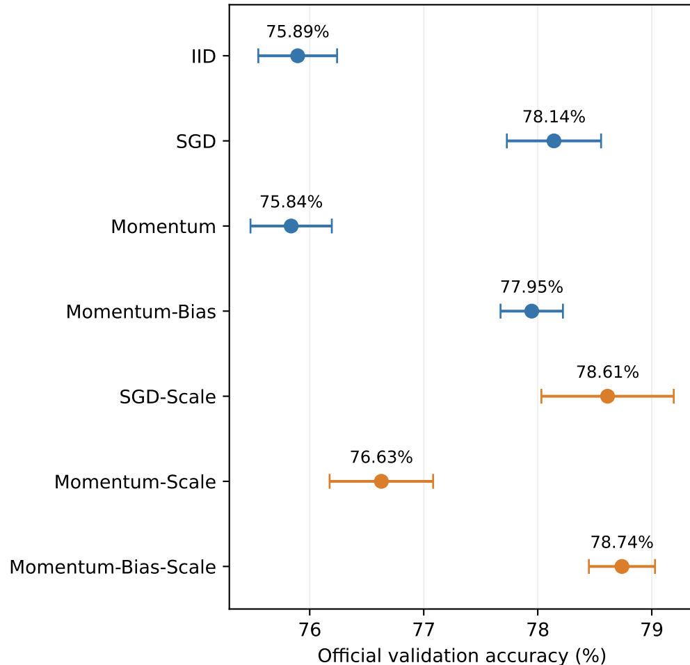
Ten shared seeds: mean and t-based 95% CI
