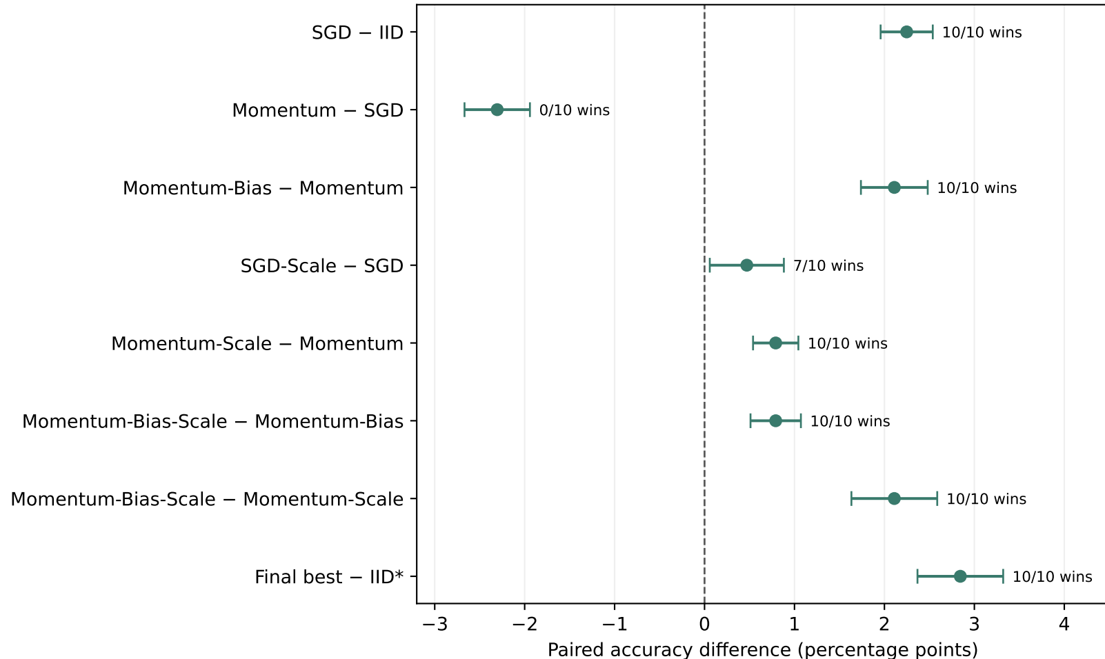
Common-seed differences: mean and 95% CI
