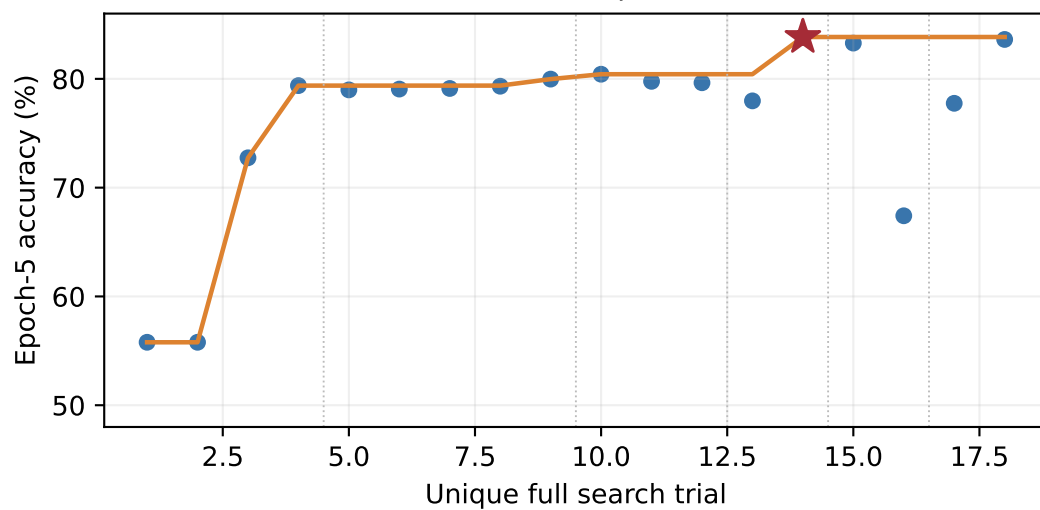
Momentum-Bias-Scale: 18/18 trials
