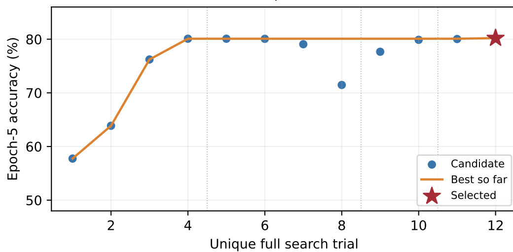
Momentum: 12/12 trials
