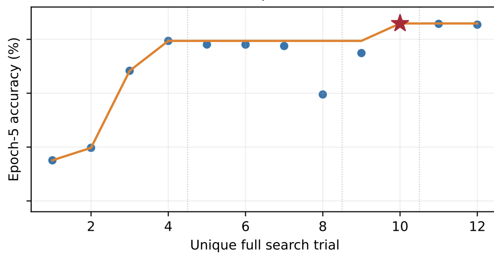
Momentum-Bias: 12/12 trials
