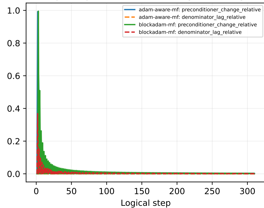
nlp: DP preconditioner changes and lag
