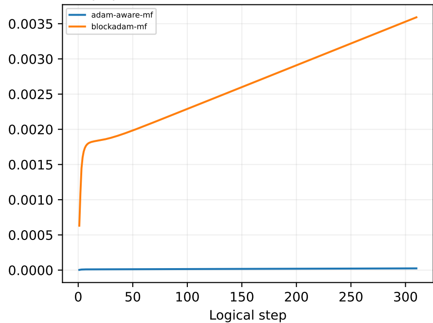
nlp: pure MF cumulative first-moment noise
