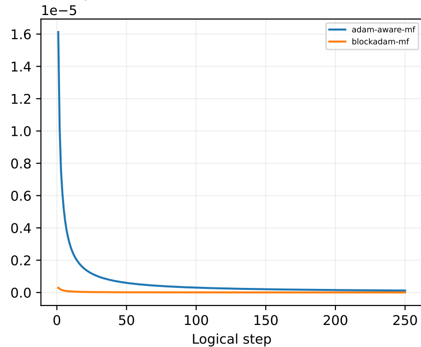
nlp: pure Gaussian second-moment variance
