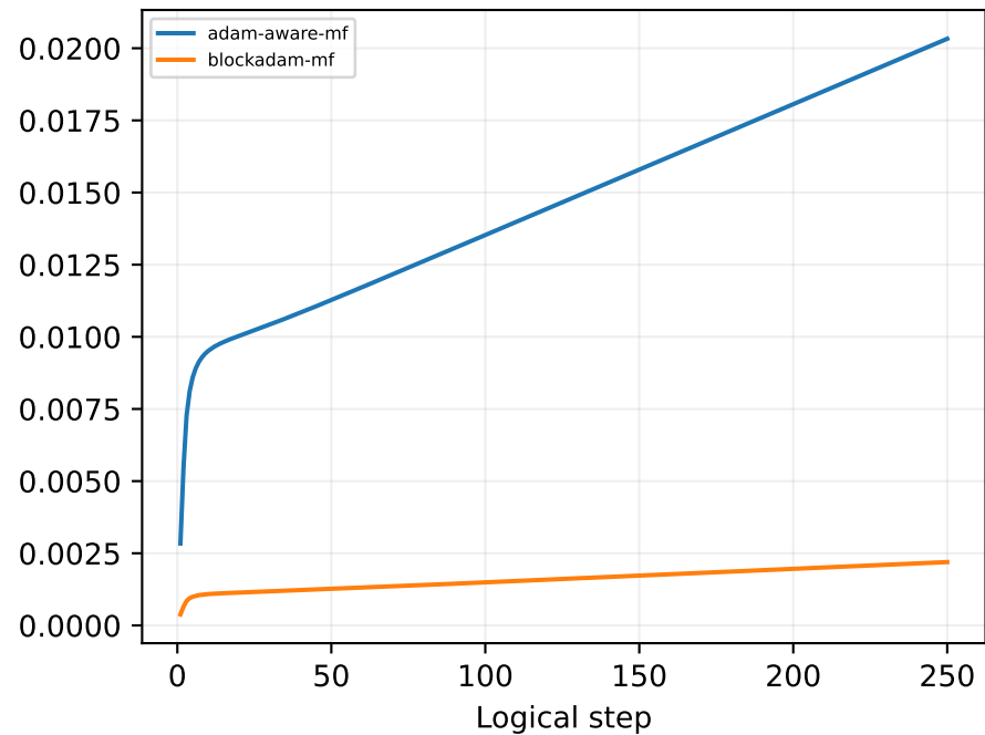
cv: pure MF cumulative first-moment noise
