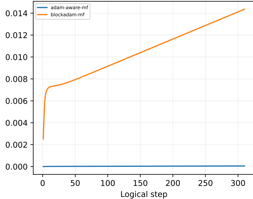
nlp: pure MF cumulative first-moment noise
