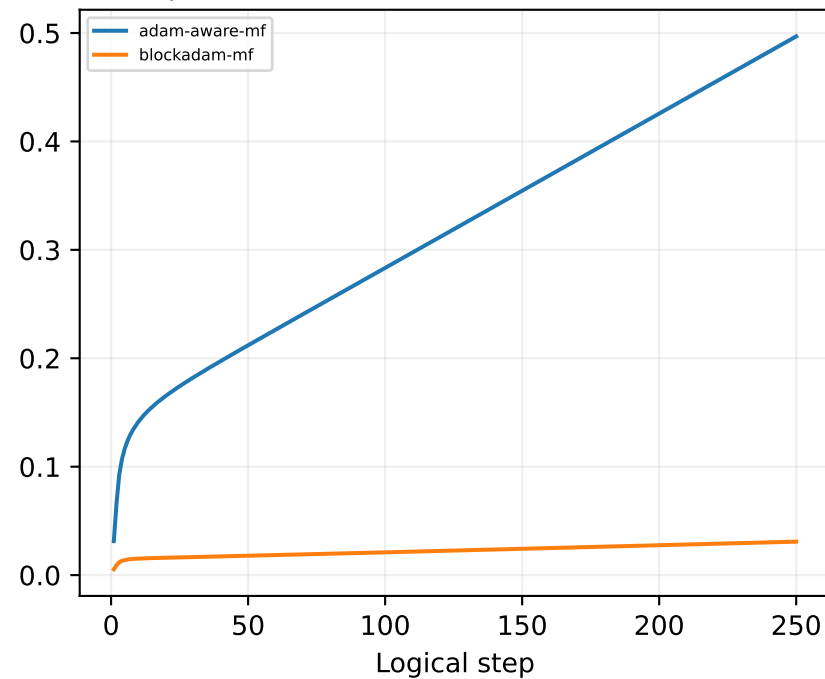
cv: pure MF cumulative first-moment noise
