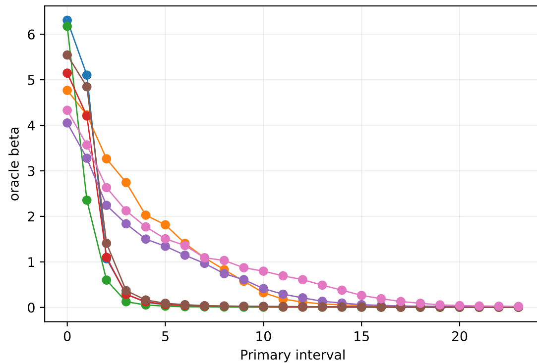
fc2
