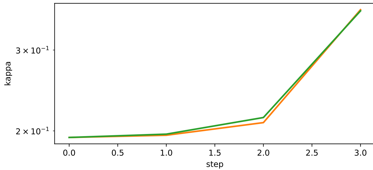
fc2
