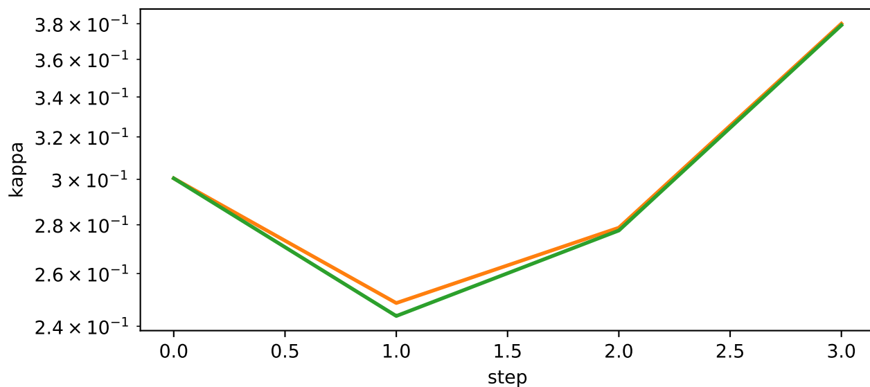
fc2
