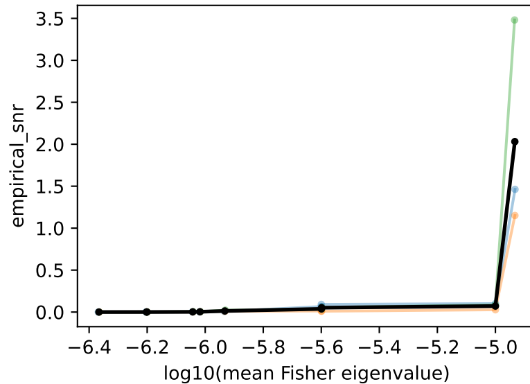
conv2; refresh 600
