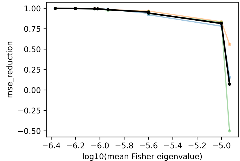
conv2; refresh 600
