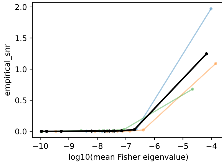
fc2; refresh 600
