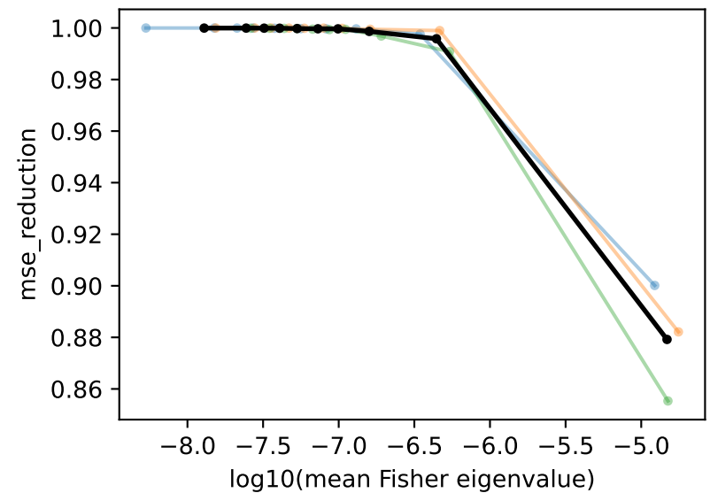
fc1; refresh 600
