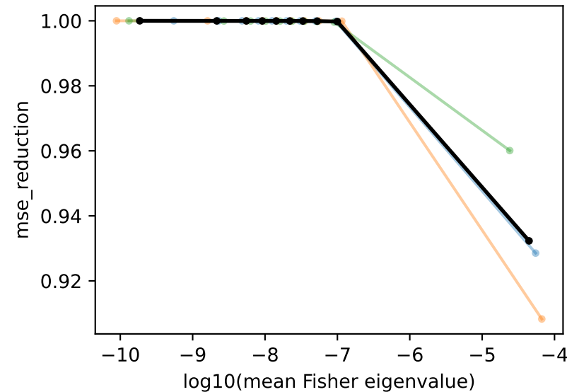
fc2; refresh 600
