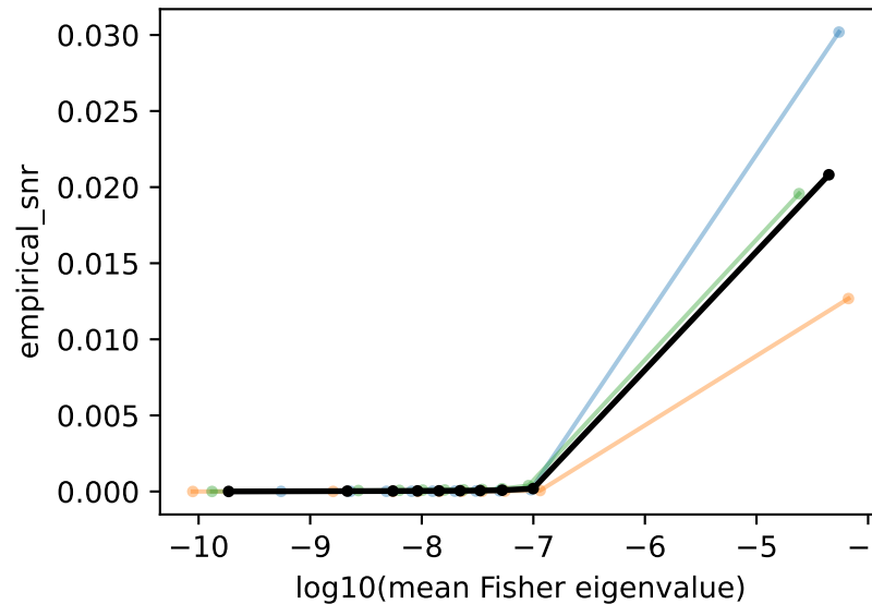
fc2; refresh 600
