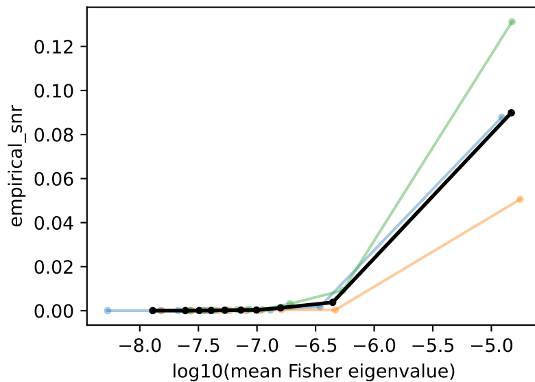
fc1; refresh 600
