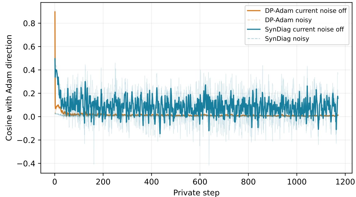
adam trajectory
