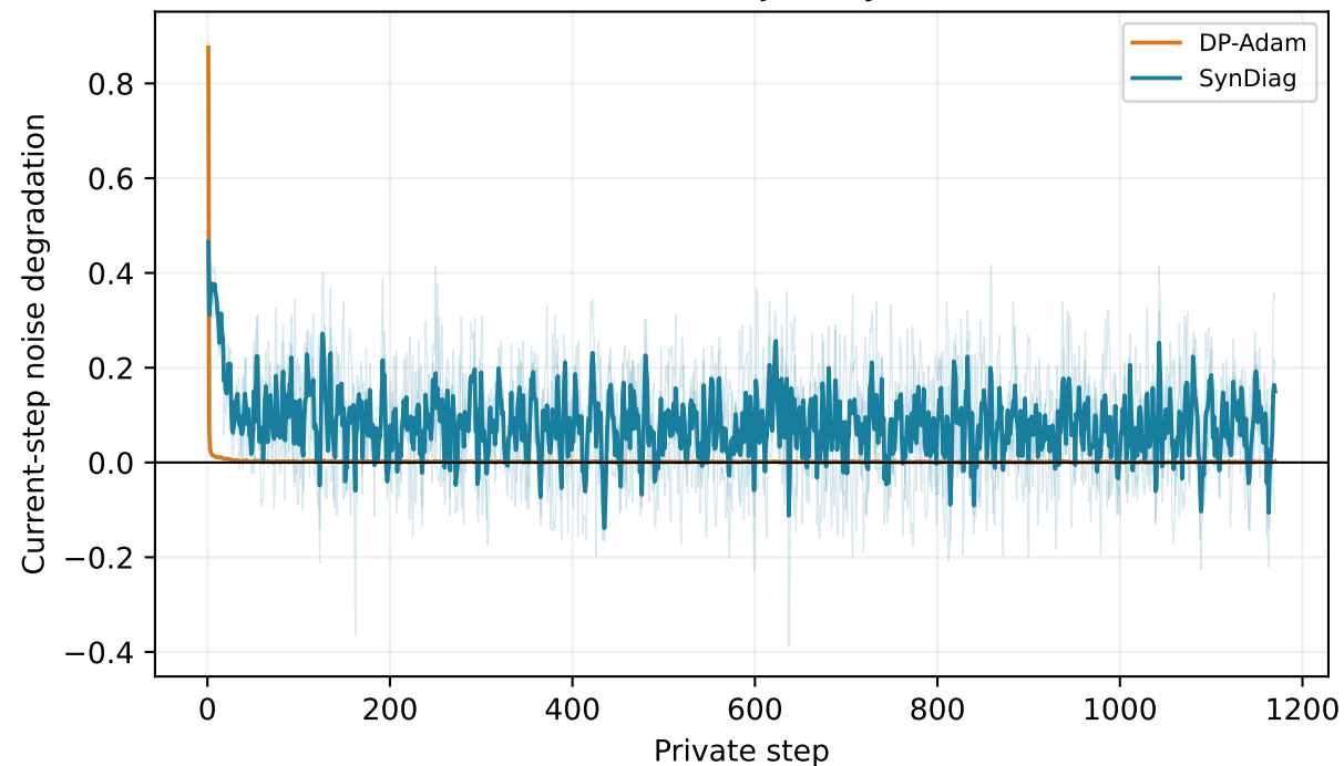
adam trajectory
