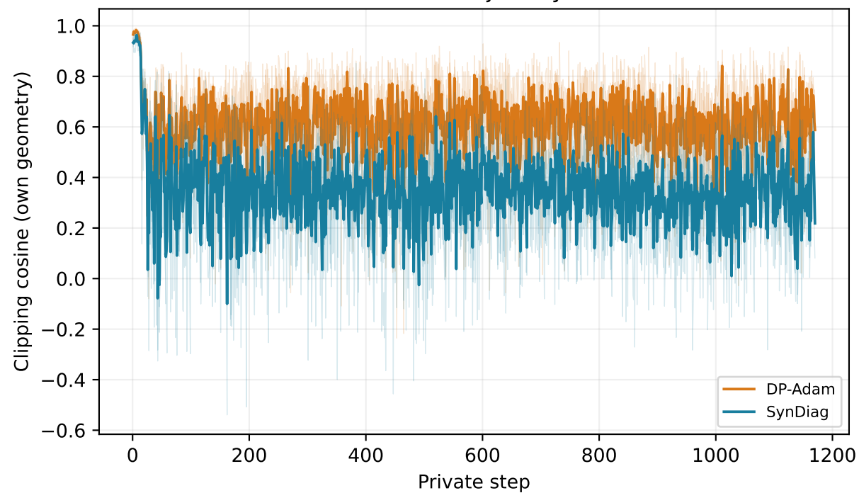
adam trajectory
