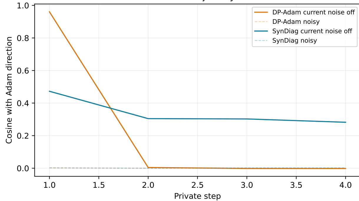
adam trajectory
