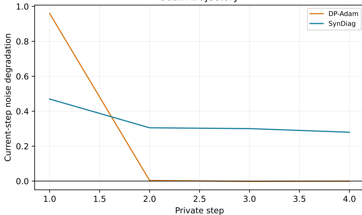
adam trajectory
