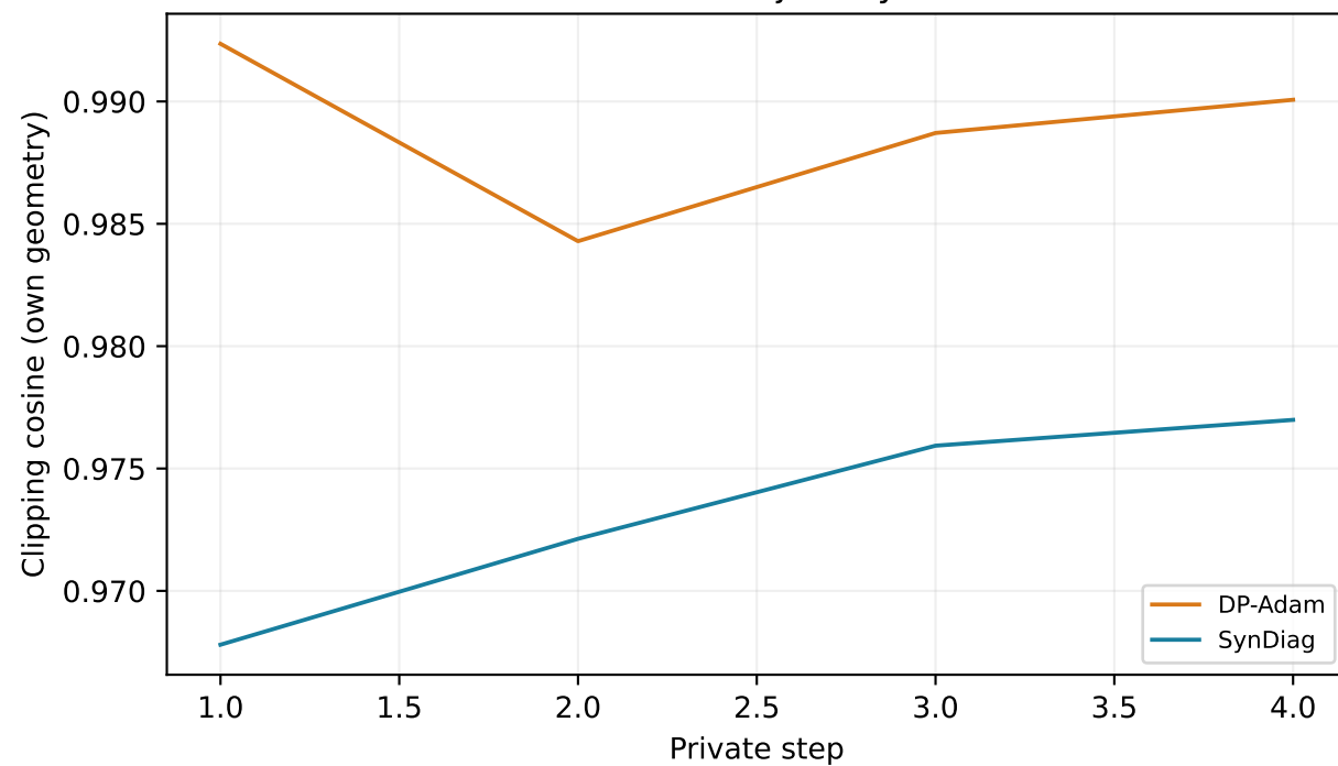
adam trajectory
