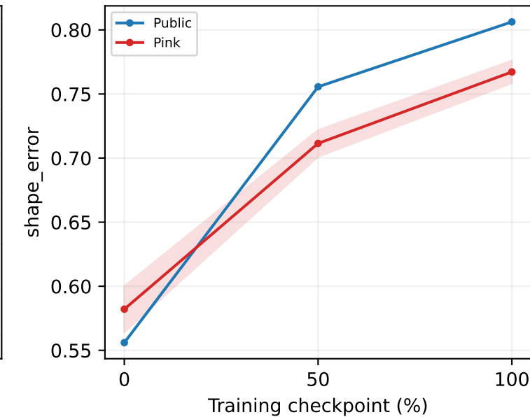
fc2
