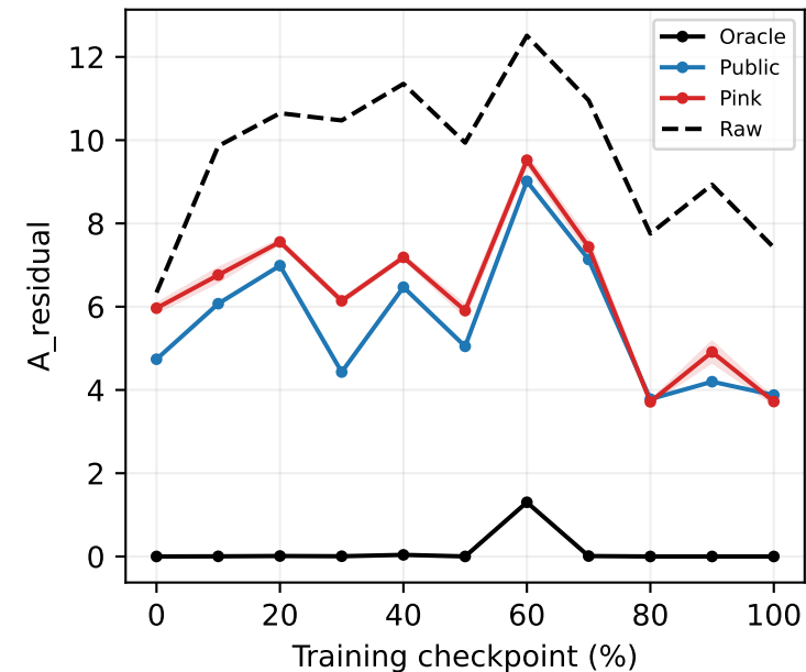
fc2
