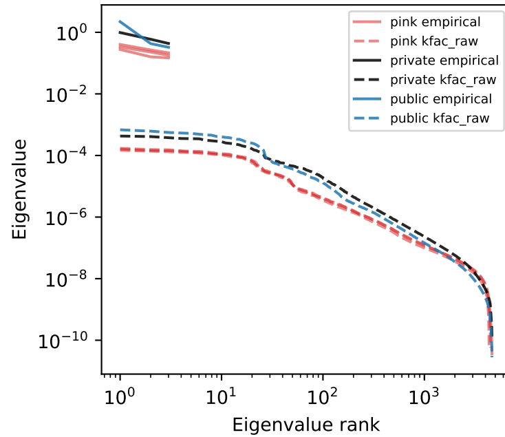
conv2 / 100%
