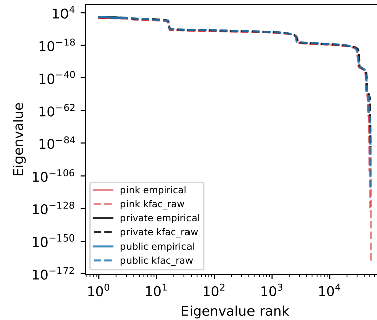
fc1 / 50%
