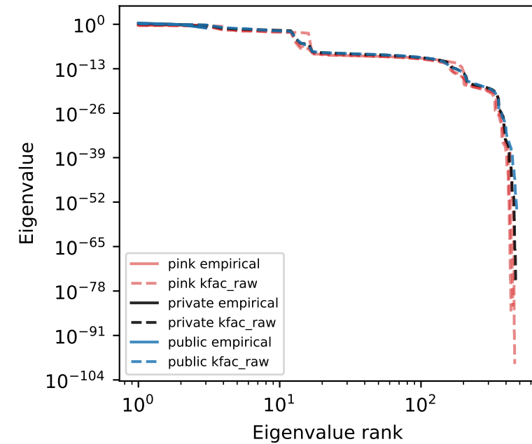
fc2 / 100%
