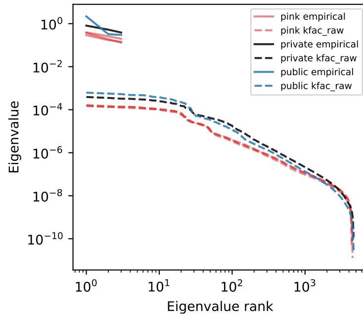
conv2 / 50%
