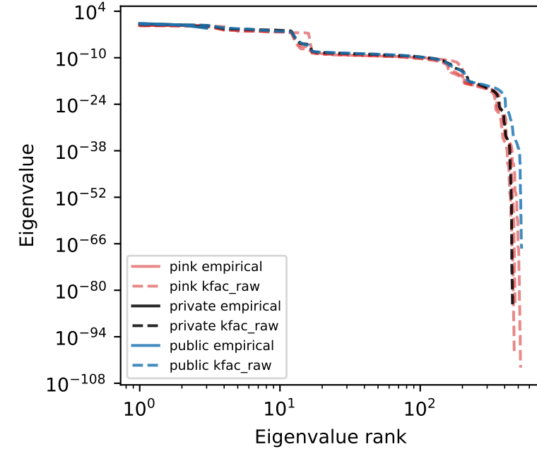
fc2 / 50%
