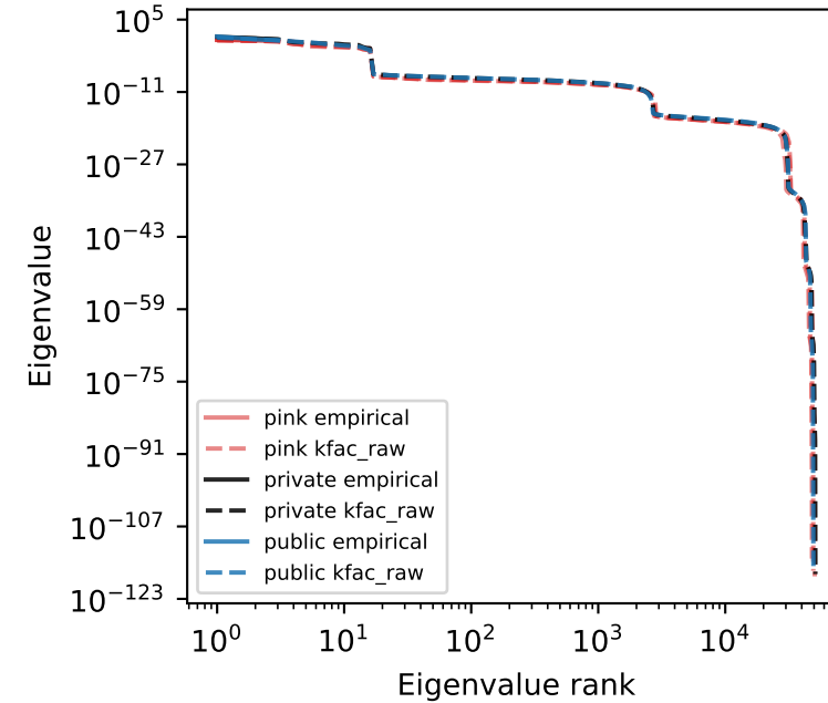
fc1 / 100%
