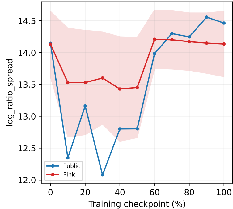
fc2
