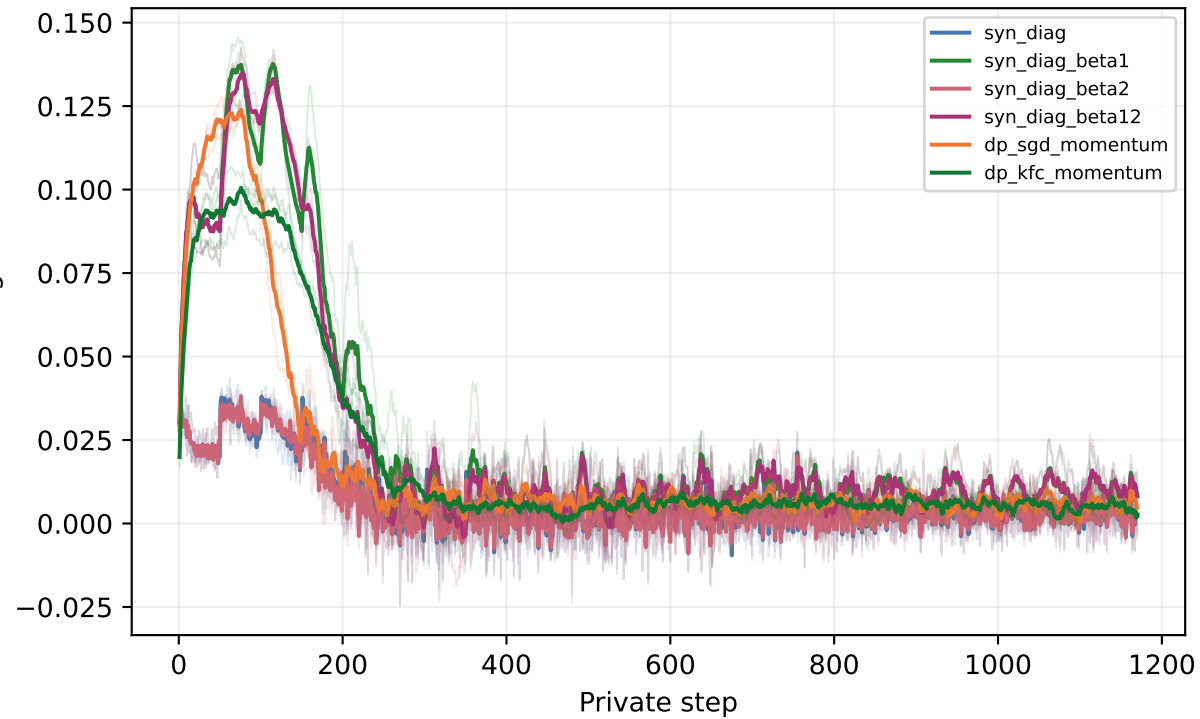
Method / Adam diagnostic cosine
