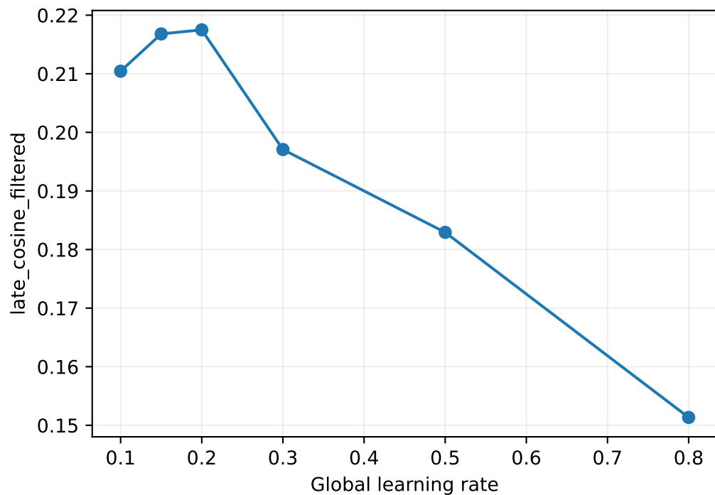
Late signal retention
