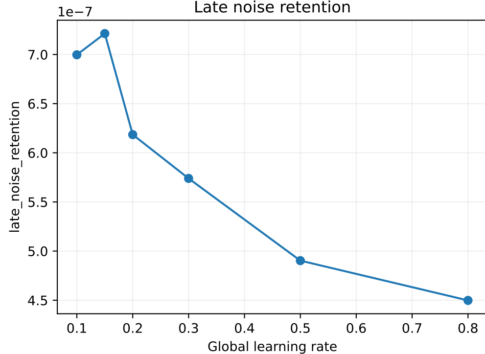
Late noise retention
