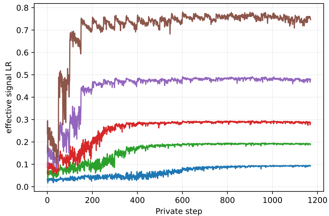
fc2
