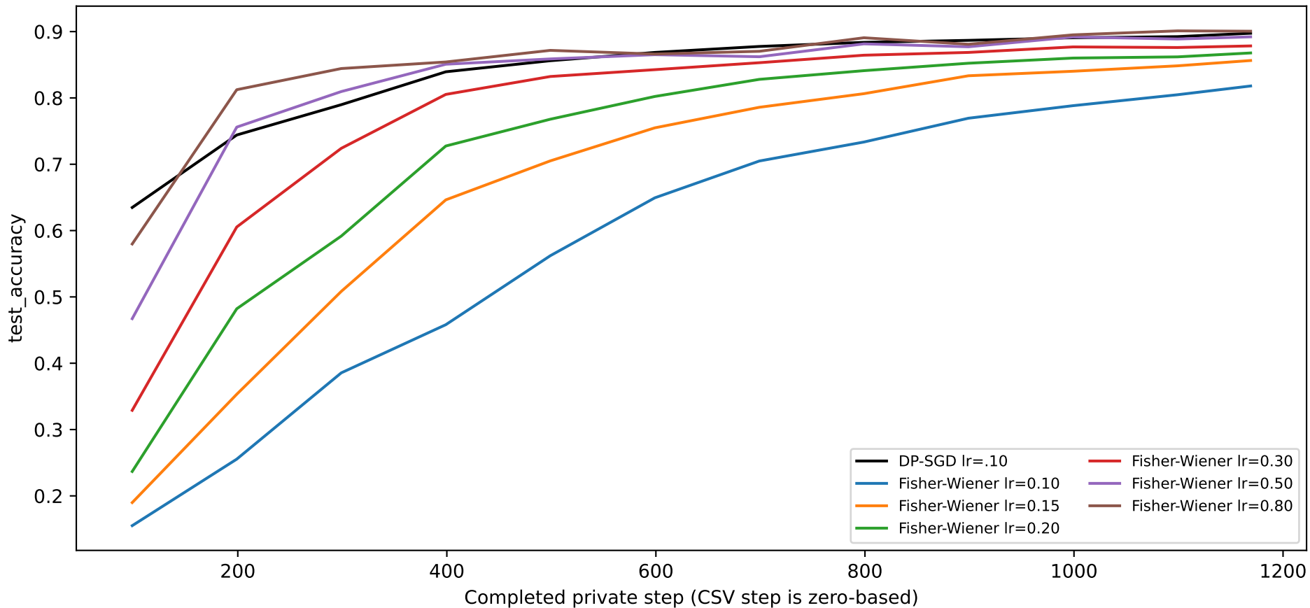
Test accuracy vs private step
