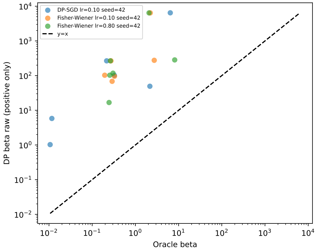
DP beta vs oracle beta
