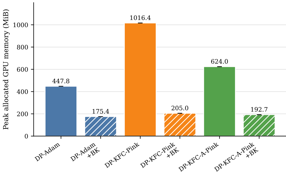
CNN-MNIST, \epsilon = 3 ; mean \pm std over 5 seeds Private training (lower is better)
