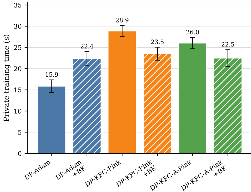
Training time (lower is better)
