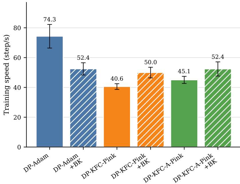
Training speed (higher is better)
