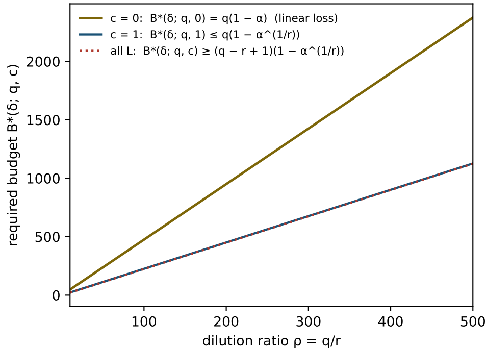
(b) Structure buys the coefficient, not the scaling ( r = 5, \alpha = \delta/D_0 = 0.05 ; Assumption 4)
