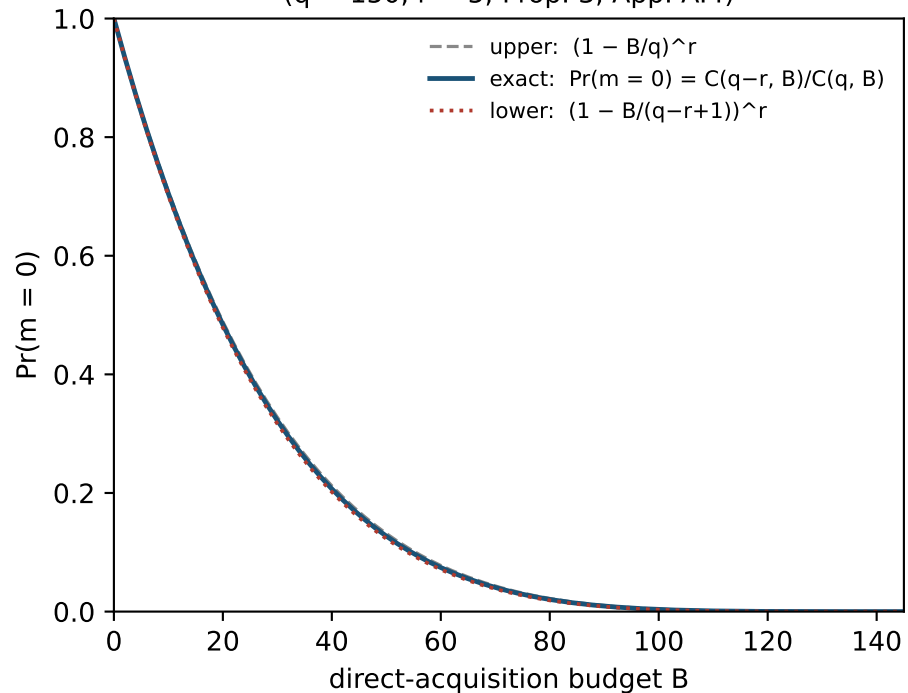
(a) Seed-failure probability and two-sided bounds ( q = 150, r = 5 ; Prop. 3, App. A.4)
