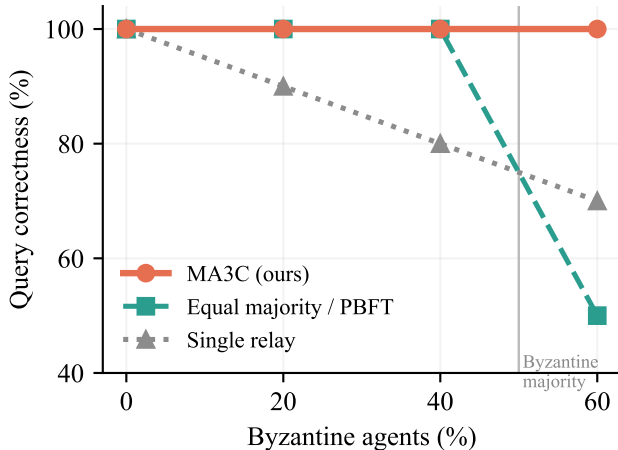
(a) Correctness
