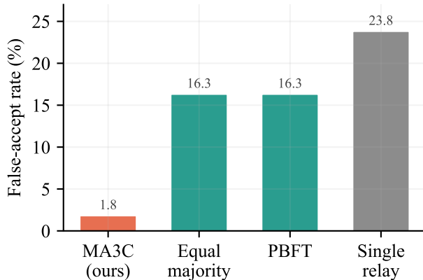
(b) Forged-evidence acceptance
