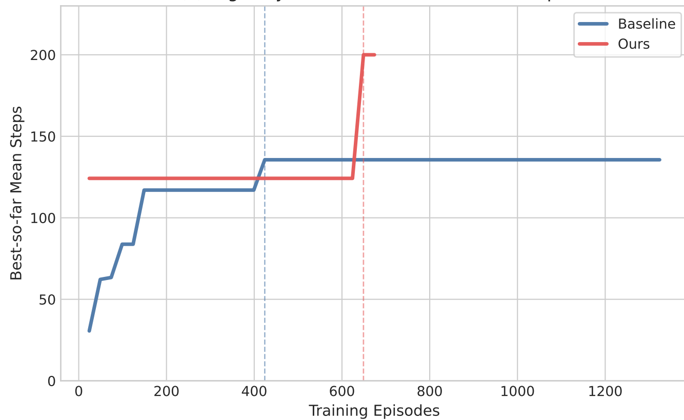
(c) Highway Standard: Best-so-far Envelope
