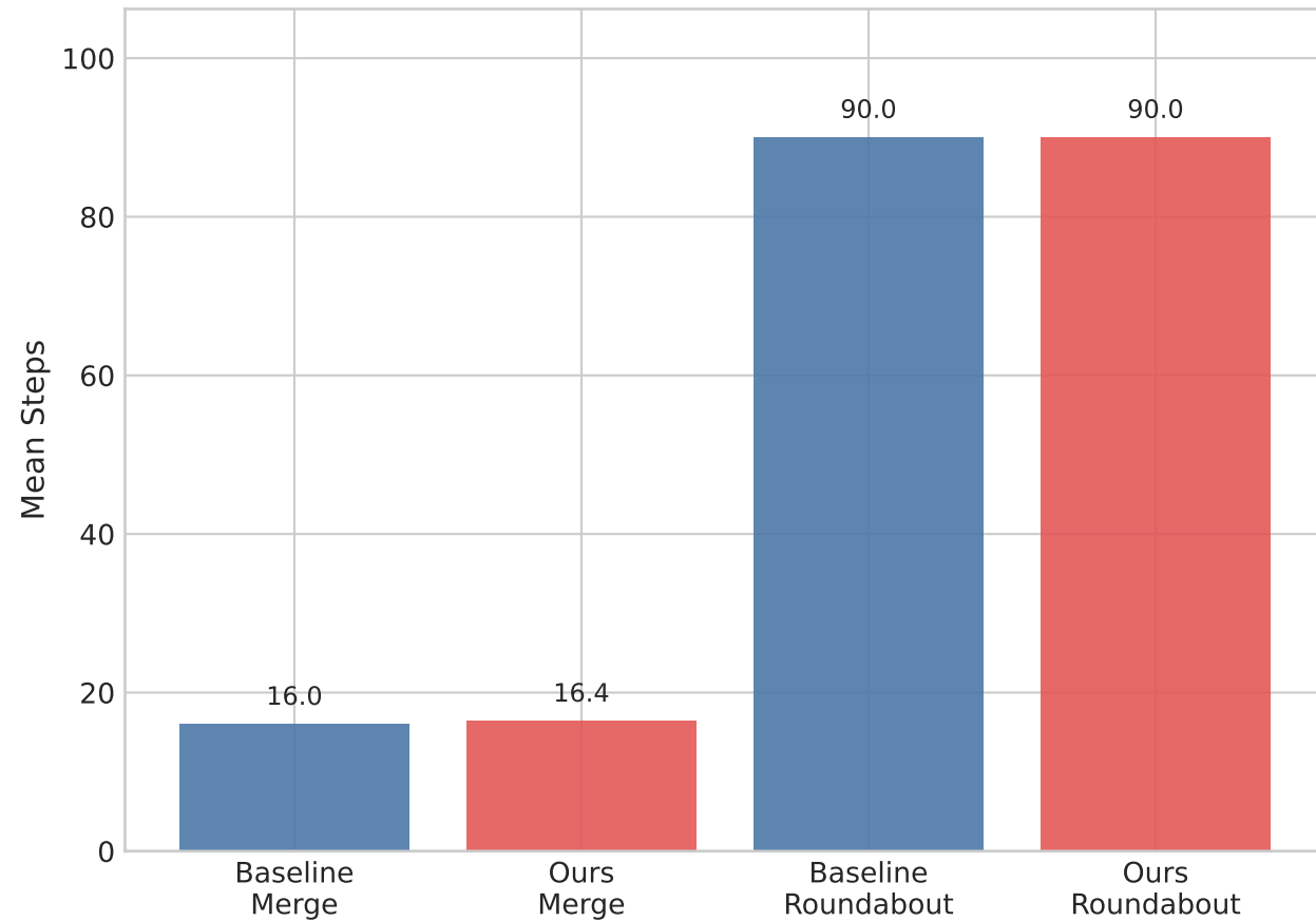
(a) Best Validation Mean Steps
