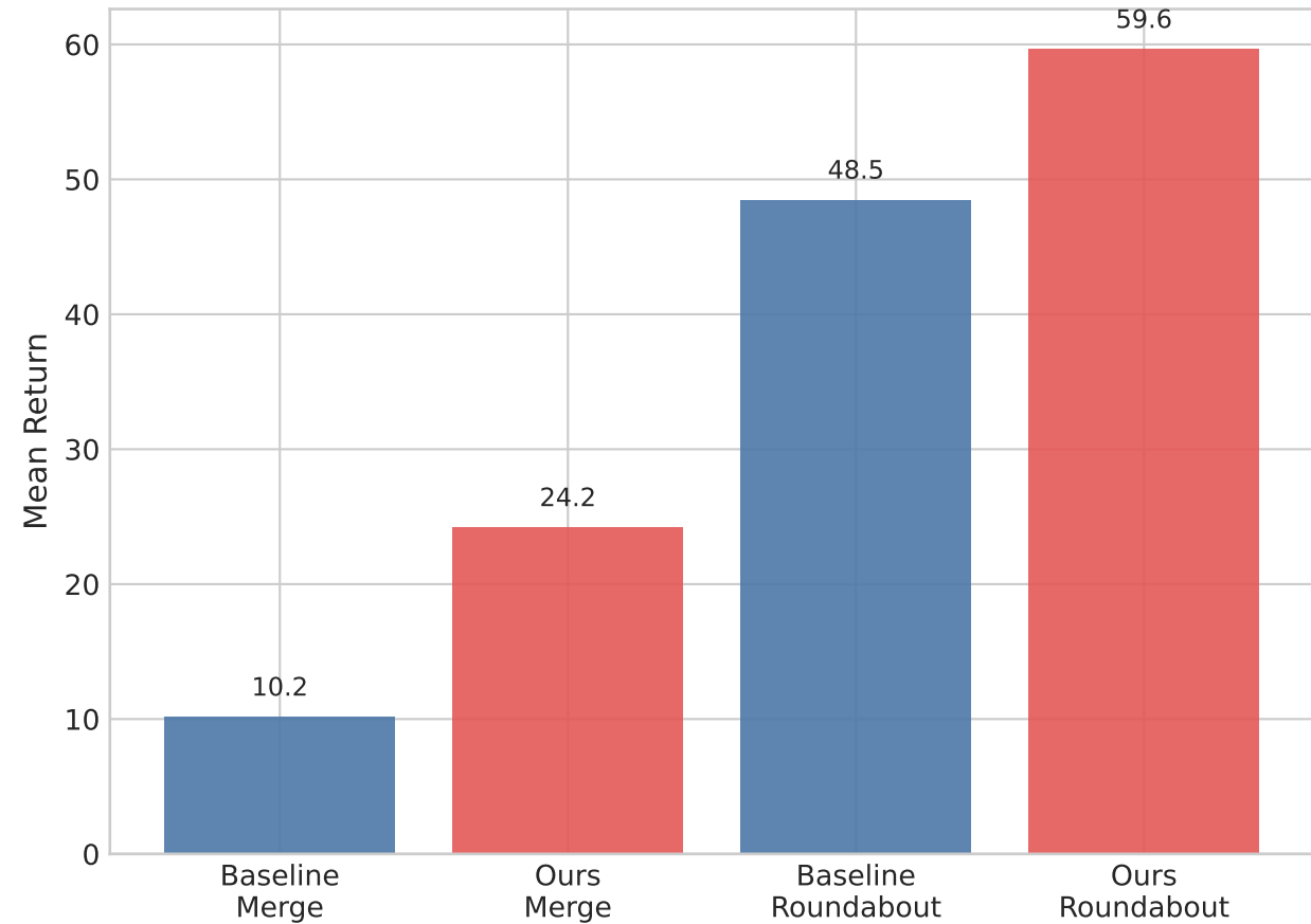
(b) Best Validation Mean Return
