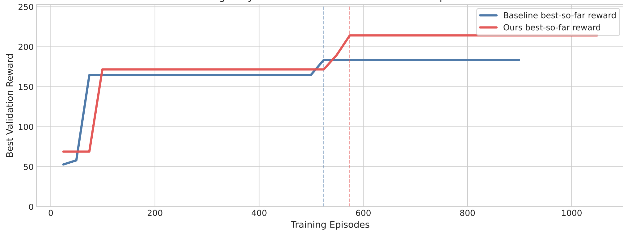
Highway Dense: Best-so-far Reward Envelope
