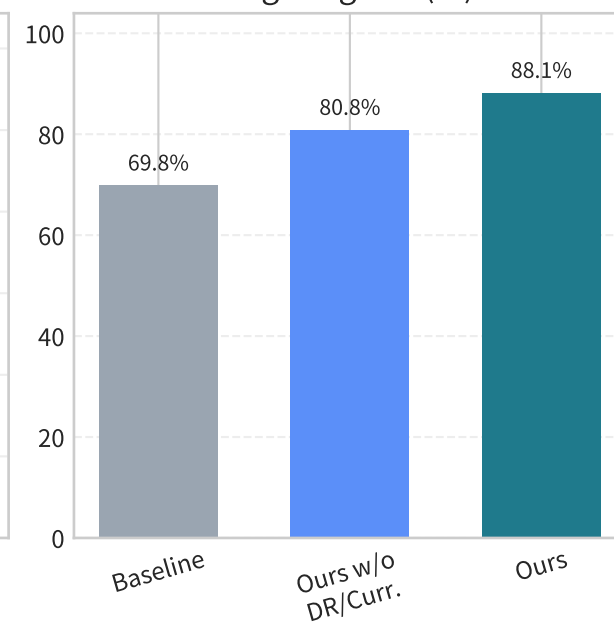
Avg Progress (%)
