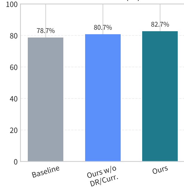
Success Rate (%)
