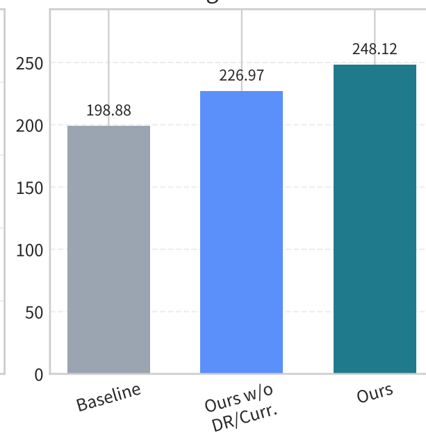
Avg Reward
