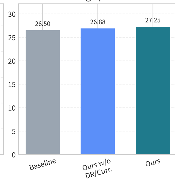
Avg Speed
