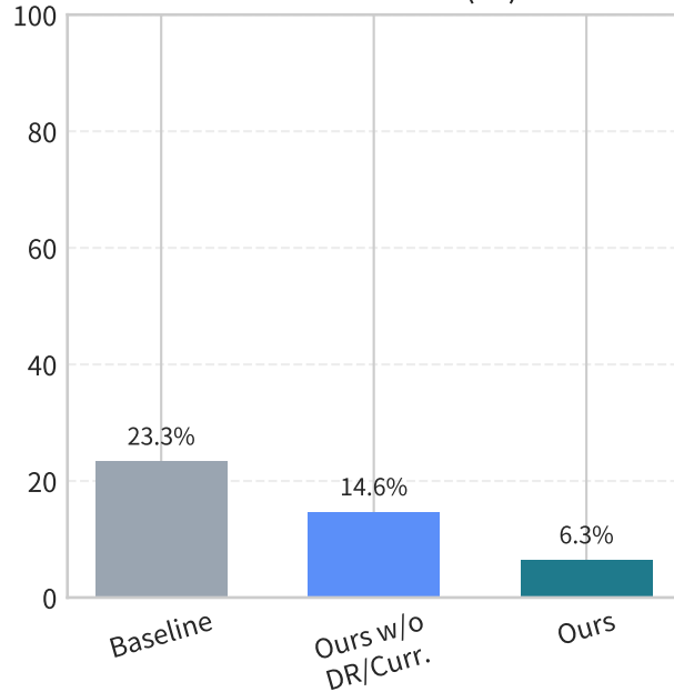
Collision Rate (%)
